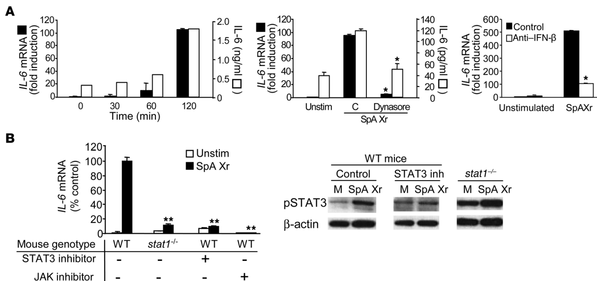
Figure 4 SpA Xr induces IFN-β- and STAT3-dependent IL-6 production. (A) Airway epithelial cells in primary culture were stimulated with SpA Xr for the times indicated or for 2 hours in the absence or presence of dynasore, and IL-6 induction was detected by real-time PCR (black bars, left y axis) or ELISA (white bars, right y axis). Untreated cells or cells stimulated with SpA Xr were incubated with IFN-β-neutralizing antibody, and IL-6 induction was measured by real-time PCR. IL-6 mRNA production is expressed as the fold induction compared with that of unstimulated cells. (B) Airway epithelial cells from WT or Stat1 -/- mice were stimulated with SpA Xr in the absence (control) or presence of the inhibitors indicated, and IL-6 production was measured by real-time PCR. IL-6 induction is expressed as a percentage of that induced by SpA Xr in cells from WT mice. (A and B) Data represent the mean and SD of 3 wells from 1 representative experiment out of 3. * P < 0.05; ** P < 0.001, Student's t test performed on the raw data. Immunoblots demonstrating phosphorylation of STAT3 in airway cells from Stat1 -/- mice and inhibition in the presence of STAT3 inhibitor are shown in B.
